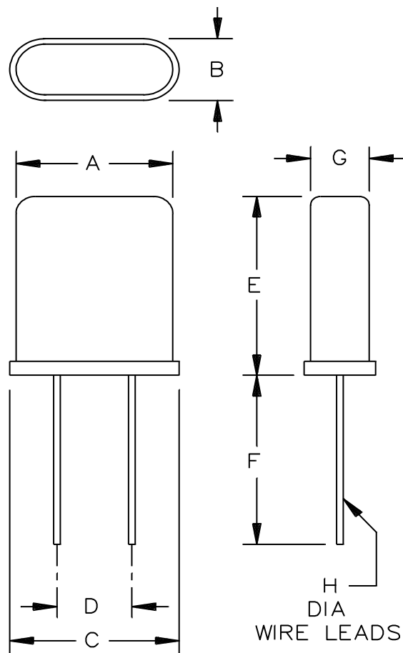
FIGURE 1. Crystal unit - CR105/U.
