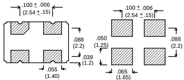
Typical PCB Layout
