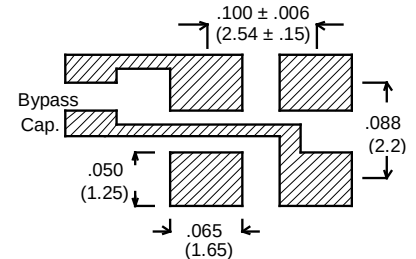
Typical PCB Layout
