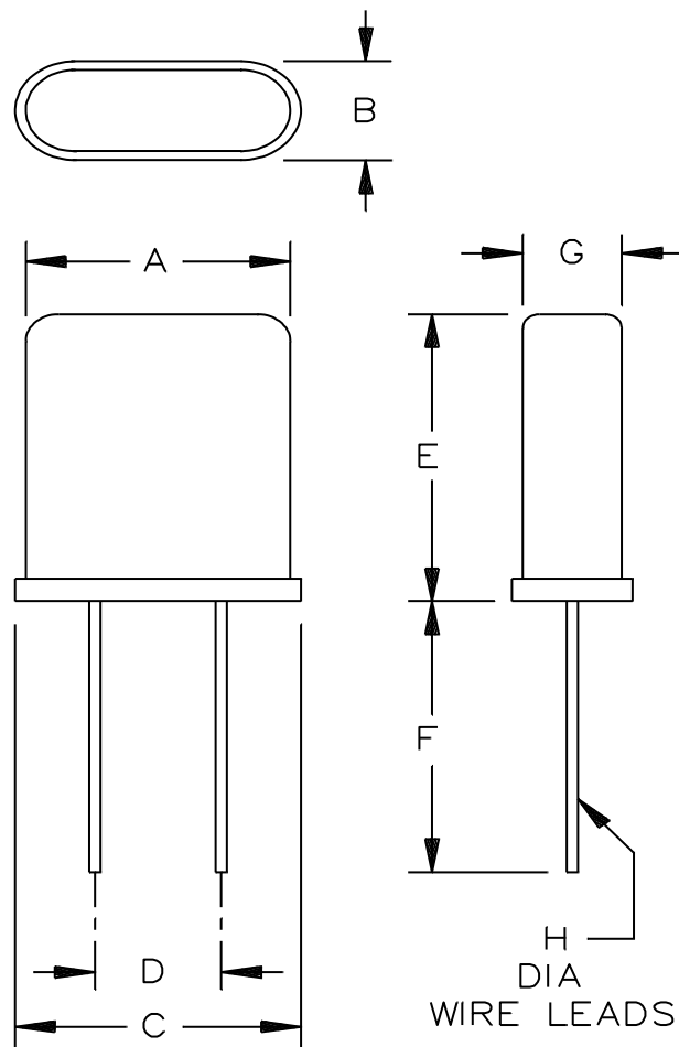
FIGURE 1. Crystal unit - CR110/U.
