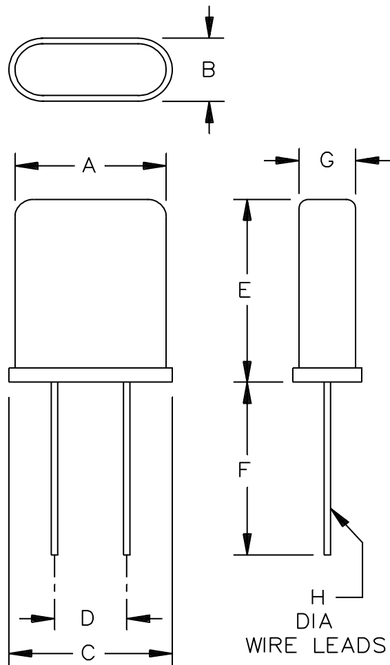
FIGURE 1. Crystal unit - CR107/U.
